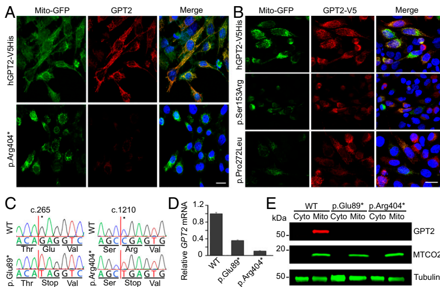
Fig. 3. GPT2 localizes to mitochondria. (A) HeLa cells coexpressing Mito-GFP (a mitochondrial marker, green) and either normal, human GPT2 (hGPT2-V5His) or human GPT2 with the p.Arg404* mutation were immunostained with anti-GPT2 antibody (red). Under the same imaging parameters, p.Arg404* showed a decrease in protein expression level. Immunostaining for GPT2 showed high colocalization with mitochondrial markers for control protein. (B) HeLa cells coexpressing Mito-GFP and C-terminal V5-tagged human GPT2 control (hGPT2-V5His) or mutations p.Ser153Arg or p.Pro272Leu were stained with anti-V5 antibody (red). Under the same imaging parameters as control, the images of cells expressing mutant GPT2 demonstrate reduced protein levels yet maintain mitochondrial localization in the residual signal. (Scale bar, 10 \mu m.) (C–E) GPT2 -mutant HEK293FT cells were generated by CRISPR-Cas9 genome editing. (C) Sanger sequencing traces of WT HEK293FT cells and the GPT2 -mutant HEK293FT cell lines are shown. The mutant cell lines harbor homozygous nonsense mutations in the GPT2 gene (c.265G>T, p.Glu89*; c.1210C>T, p.Arg404*). Positions of the variants are according to NM_133443.3 (cDNA) and NP_597700.1 (protein). (D) Graphed are the results of qRT-PCR analysis of WT HEK293FT cells and the two lines of GPT2 -mutant cells (p.Glu89*, p.Arg404*). For all samples, GPT2 mRNA was normalized to 18S rRNA. (E) Immunoblot analysis of WT HEK293FT cells and the GPT2 mutant cells (p.Glu89*, p.Arg404*). In WT cells, GPT2 is absent from the cytosolic fraction (Cyto) and highly enriched in the mitochondrial fraction (Mito). In cells expressing either of the two mutants, GPT2 is absent from both fractions. Tubulin and MTCO2 (cytochrome c oxidase subunit II) are shown as a loading control marker and a mitochondrial marker, respectively.
